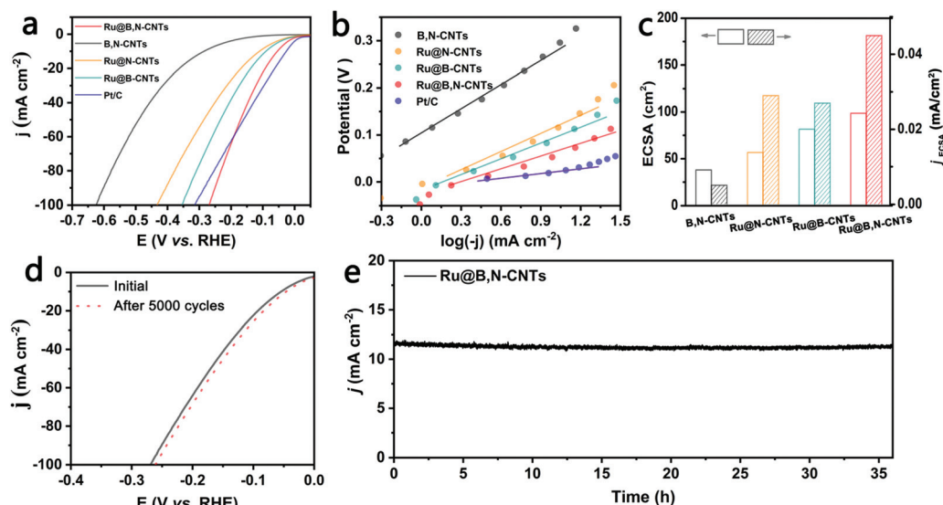
Fig. 4 (a) The linear sweep voltammetry (LSV) curves for the HER of B,N-CNTs, Ru@B-CNTs, Ru@N-CNTs, Ru@B,N-CNTs and commercial Pt/C in a 1 M KOH solution. (b) The Tafel plots for the electrocatalysts. (c) Comparison of ECSAs and the current density produced at a fixed overpotential of 0.1 V (normalized by the ECSAs). (d) The LSV curves obtained for HER over Ru@B,N-CNTs before and after 5000 cycles of CV scans. (e) The chronoamperometric i - t curve for 36 h.
