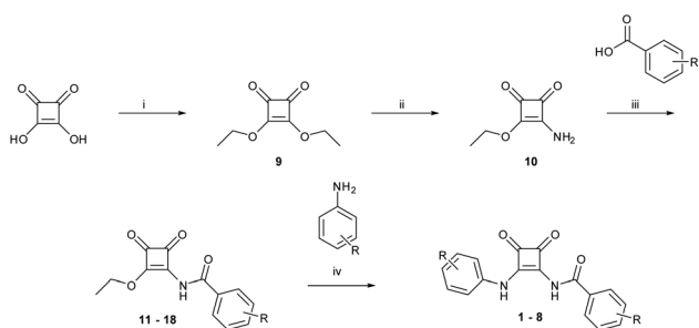
Scheme 1 Synthetic pathway to amido-squaramides. Reagents and conditions: (i) triethyl orthoformate, EtOH, 80 °C, 72 h, 91%; (ii) 20% ammonium carbonate in ethanol, EtOH, rt, 18 h, 70%; (iii) EDCI-HCl, DMAP, MeCN/DMF (anhydrous), \text{N}_2 , rt –80 °C, 18 h, 10–83%; (iv) \text{Zn}(\text{OTf})_2 , MeCN/DMF, 80 °C, 3–18 h, 10–71%.
