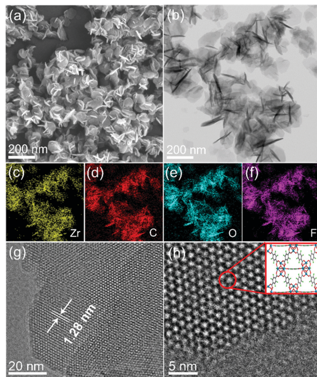
Fig. 1 (a) SEM, (b) TEM, (c)–(f) EDS mapping, (g) high-resolution TEM, and (h) STEM iDPC images (inset shows the corresponding structure) of UiO-66- F_4 .
