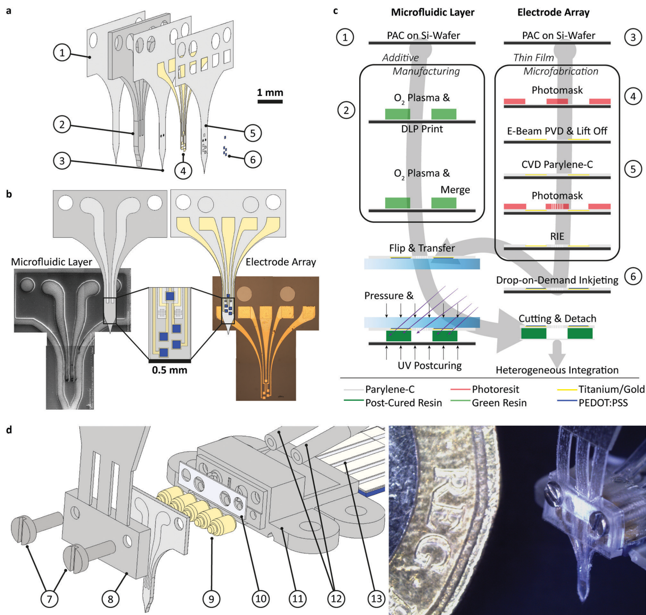
Fig. 1 Hybrid fabrication of the multimodal intracranial implant: (a) exploded view of the implant (1 to 6) and assembled headstage for acute in vivo experiments (7 to 13): 1 bottom PAC layer (2 \mu m), 2 3D printed, flexible body with microfluidic system (200 \mu m), 3 middle PAC layer (2 \mu m) with \mu -fluidic in- and outlet, 4 10 nm titanium-100 nm gold electrodes, 5 top PAC layer (2 \mu m) with etched \mu -fluidic in- and outlets as well as electrical contacts, 6 Drop-on-demand inkjet-printed PEDOT:PSS layer (77 \pm 11 nm), 7 fastener M0.6 \times 5 mm, 8 3D printed socket for acute in vivo experiments, 9 pogo pins, 10 medical-grade double-sided adhesive tape (85 \mu m), 11 3D printed fluidic and electric interface with M0.6 thread, 12 1/32" polyethylene tubing (0.8 mm OD, 0.4 mm ID) and 13 tailored FPC cable (5 ways, 1 mm pitch); (b) left: technical drawing and SEM picture of 3D printed body showing the \mu -fluidic channels (top view) and right: technical drawing and optical micrograph of the Au layer (top view). (c) Convergent hybrid fabrication schema, combining additive manufacturing and thin-film microfabrication; (d) exploded view and microscopy picture of the assembly.
