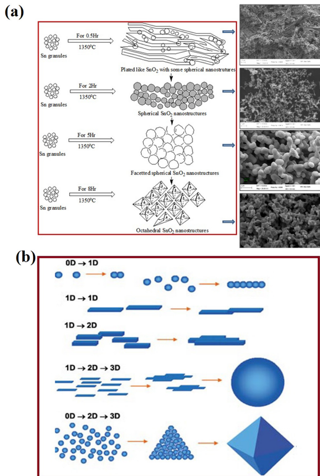
Fig. 7 (a) Schematic of the \text{SnO}_2 structural growth phenomena and morphological transformation with increasing evaporation time during thermal evaporation at 1350 °C. Reprinted with permission from ref. 152. Copyright 2014 Elsevier. (b) Various organizing schemes for the self-construction of nanostructures by oriented attachment. Reprinted with permission from ref. 151. Copyright 2004 John Wiley and Sons.
