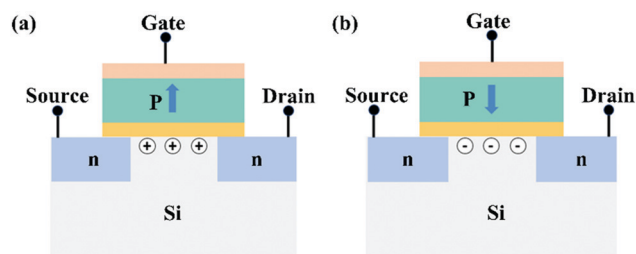
Fig. 6 Structure schematic diagram of the N-channel enhanced MFMIS-type FeFET: (a) the transistor is in the off state; (b) the transistor is in the on state.
