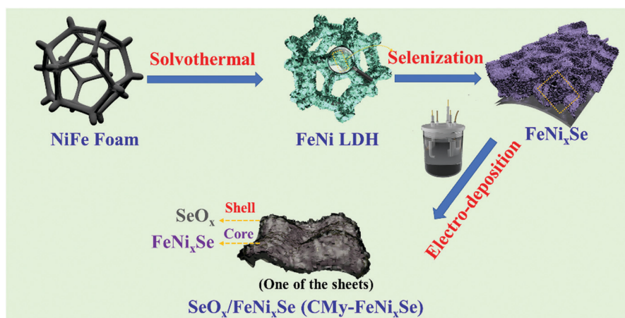
Scheme 1 Schematic illustration of the formation process of hierarchical \text{SeO}_x/\text{FeNi}_x\text{Se} (CM y -FeNi x Se).
