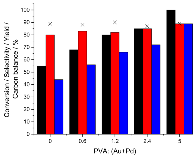
Fig. 3 Effect of PVA: metal ratio on catalytic activity of the 0.33%Au–0.33%Pd/TS-1 catalyst activity towards the ammoximation of cyclohexanone oxime via in situ H_2O_2 synthesis. Ammoximation reaction conditions: cyclohexanone (2 mmol), NH_4HCO_3 (4 mmol), 5% H_2/N_2 (420 psi), 25% O_2/N_2 (160 psi), catalyst (0.075 g), t -BuOH (5.9 g), H_2O (7.5 g), 3 h, 80 °C 800 rpm. Key: cyclohexanone conversion (black bar), selectivity towards oxime (red bar), cyclohexanone oxime yield (blue bar), carbon balance (crosses). Note: all catalysts were exposed to an oxidative heat treatment prior to use (static air, 400 °C, 3 h).
