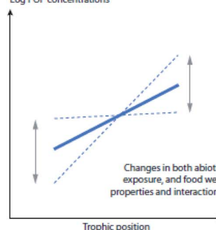
Fig. 1 Conceptual figures showing the concentrations of POPs in relation to trophic position, in the case that climate change influences (top) food web properties or interactions, (middle) abiotic exposures, or (bottom) both food web properties/interactions and abiotic exposures. The solid line represents the present log-normal relationship between the trophic position of the organisms and accumulated contaminant concentrations, while dotted lines reflect the projected window of biomagnification because of the influence of climate change. NAO = North Atlantic Oscillation; TL = trophic level.
