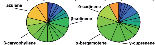
Fig. 5 Composition weighted hydroxyl reactivity of sesquiterpene species identified and quantified at the tower and farm sites. The top three sesquiterpene contributors to hydroxyl reactivity for each site are listed next to their corresponding slice.
