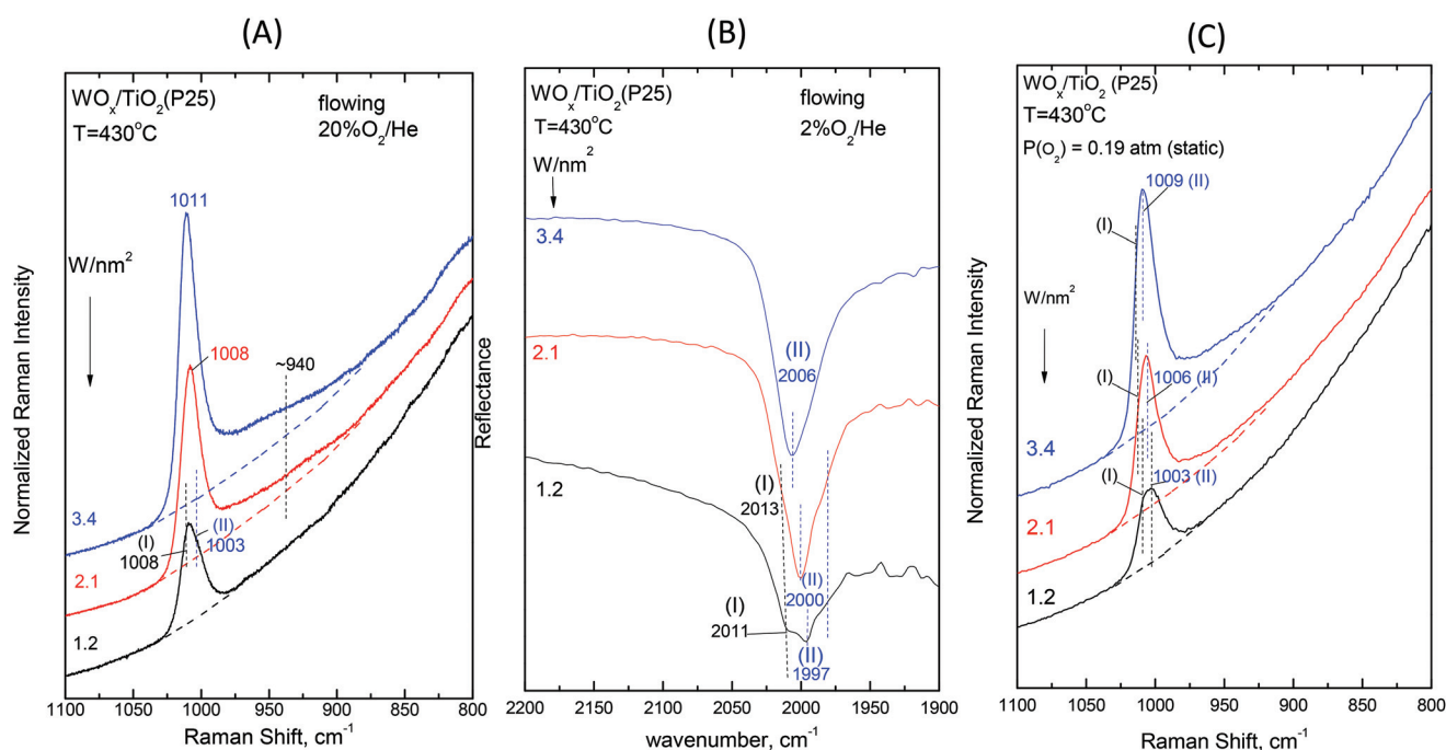
Fig. 8 Dependence on surface coverage for \text{WO}_x/\text{TiO}_2(\text{P25}) at T = 430 °C. (A) In situ Raman spectra obtained under flowing 20\% \text{O}_2/\text{He} for samples with W surface densities ( \text{W nm}^{-2} ) as indicated by each spectrum; spectral conditions: see Fig. 2(A) caption. (B) In situ FTIR spectra obtained under flowing 2\% \text{O}_2/\text{He} for samples with W surface densities ( \text{W nm}^{-2} ) as indicated by each spectrum. (C) Raman spectra at static equilibrium under p_{\text{O}_2} = 0.19 atm for samples with W surface densities ( \text{W nm}^{-2} ) as indicated by each spectrum; spectral parameters: see Fig. 2(C) caption.
