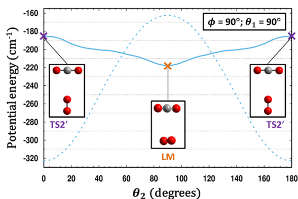
Fig. 6 A comparison is made between the PESs of CO_2 - O_2 (solid line) and CO_2 - N_2 (dashed line). 35 For each system, a scan of \theta_2 is performed holding \theta_1 and \phi fixed, and for each value of \theta_2 , the energy in each case is minimized with respect to R . Remarkably, what is a T-shaped global minimum for CO_2 - N_2 becomes an unstable 2nd-order saddle in CO_2 - O_2 , while the cross-shaped structure in the center of the plot at \theta_2 = 90^\circ is a local minimum for CO_2 - O_2 yet a transition structure for CO_2 - N_2 .
