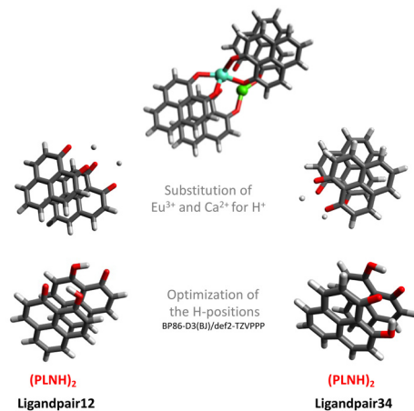
Fig. 7 Starting from the M1-D3 structure of [Eu(PLN) 4 Ca] + calculated at the BP86-D3(BJ)/def2-TZVPP level, this scheme describes the definition of the models (Ligandpair12 and Ligandpair34) used for benchmarking the dispersion interactions in this type of complexes (europium: clear blue; calcium: green; oxygen: red).
