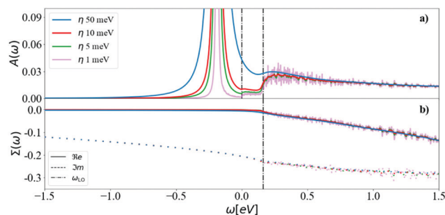
Fig. 6 The (a) spectral function and (b) self-energy at the CBM and 300 K calculated using DM and a N = 128 for different values of \eta = 50, 10, 5 and 1 meV. The first vertical line is at 0 energy (CBM) and the second at the highest phonon frequency. The finite temperature allows for absorption of acoustic phonons, which produces a small plateau between the QP peak and the main (optical) satellite feature.
