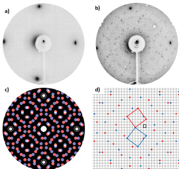
Fig. 3 LEED pictures acquired with a beam energy of 55 eV on (a) the Fe- p(1 \times 1)\text{O} and (b) the 1 ML VOTPP/Fe- p(1 \times 1)\text{O} surface. (c) LEEDpat simulation of the expected LEED pattern for the (5 \times 5) R37 1 ML VOTPP superstructure. (d) Real space schematics of the corresponding two molecular domains formed on top of the substrate. The VOTPP lattice unit cell (red and blue rectangles represent the two possible orientations) is 5 \times 5 times larger than the substrate one (black grid).
