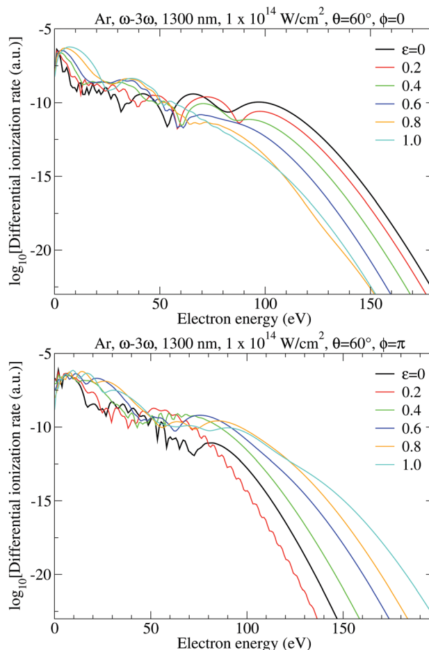
Fig. 10 The logarithm of the differential ionization rate of Ar atoms as a function of the photoelectron energy in electron volts for ionization by an \omega - 3\omega BEOTC field with the ellipticities \varepsilon = \varepsilon_1 = \varepsilon_2 as indicated. Both the direct and the rescattered electrons are included. The intensities of the field components are I_1 = I_2 = 1 \times 10^{14} \text{ W cm}^{-2} , the fundamental wavelength is 1300 nm, and the emission is in the direction \theta = 60^\circ . The relative phase is \phi = 0 (upper panel) and \phi = \pi (lower panel).
