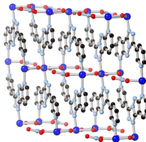
Fig. 12 The extended structure of the copper(II) coordination polymer containing L14 reported by Li and co-workers. 60 Copper atoms coloured dark blue.
