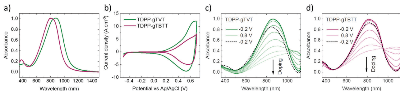
Fig. 1 (a) Normalized UV-Vis-NIR absorption spectra and (b) cyclic voltammograms of the polymer films spin-cast from chloroform on ITO substrates. The CV curves were recorded with a scanning speed of 80 \text{ mV s}^{-1} in aqueous NaCl solution (0.1 M). The 10th cycle is shown. (c and d) UV-Vis absorption spectra of the films during the forward doping sweep ( -0.2 \text{ V} to 0.8 \text{ V} ) direction and as they were de-doped (black dashed spectrum, at -0.2 \text{ V} ). All measurements were performed in aqueous NaCl solution (0.1 M) and voltages were applied vs. Ag/AgCl. The film thickness was in the range of 80–125 nm.
