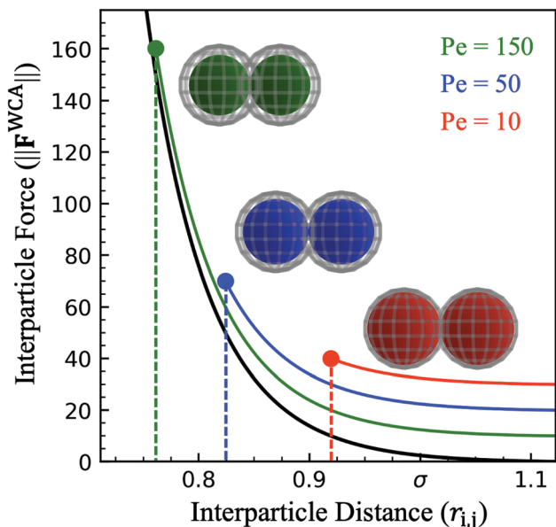
Fig. 3 Force at varying interparticle separation distance ( r_{ij} ) for the WCA potential (eqn (1), black) for constant repulsive well-depth ( \varepsilon = 0.1 ), showing sensitivity to activity. For a head-on collision of active particles ( Pe_{red} < Pe_{blue} < Pe_{green} ) points indicate the maximum particle deformation while lines indicate range of interparticle distance available in other types of collisions. Colored spheres demonstrate the maximum deformation at each activity and wire mesh overlay shows the extent of particle overlap (for particle diameter \sigma = 1.0 ).
