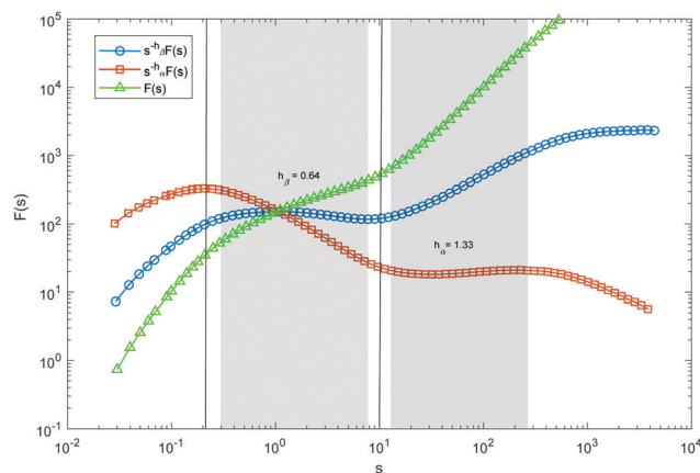
Fig. 5 Compensating plot. In this plot, we show how we derive h_\beta and h_\alpha from original data of F(s) versus s . A compensated plot of s^{-h_\beta}F(s) versus s , the blue circles, becomes flat over \beta region for h_\beta = 0.64 . Similarly, A compensated plot of s^{-h_\alpha}F(s) versus s , the brown squares, becomes flat over \alpha region for h_\alpha = 1.33 .
