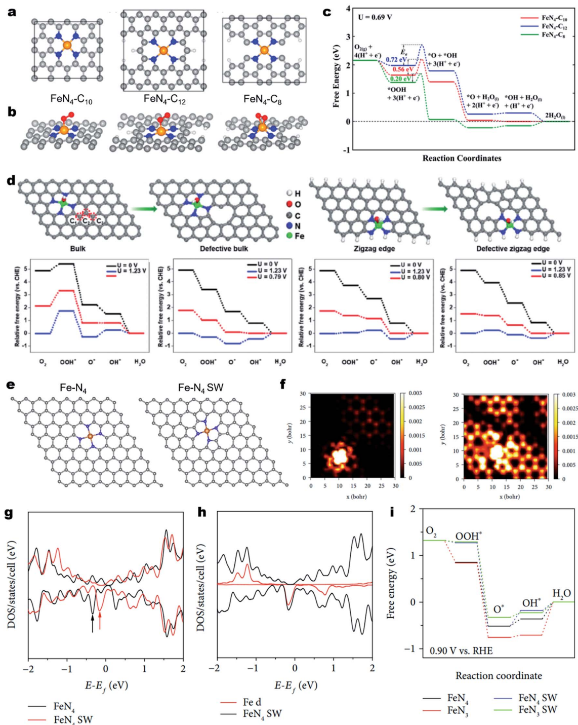
Fig. 6 Regulating the carbon skeleton geometry for enhancing the ORR activity. (a) Atomistic configuration of the \text{Fe-N}_4 moiety with different local carbon structures of \text{Fe-N}_4\text{-C}_{10} , \text{Fe-N}_4\text{-C}_{12} , and \text{Fe-N}_4\text{-C}_8 and (b) corresponding \text{O}_2 adsorption configuration. (c) Calculated free energy diagrams for the ORR through an OOH dissociation pathway on the above three different active sites under a potential of 0.69 V in acidic medium. Reproduced with permission from ref. 160. Copyright (2017) American Chemical Society. (d) Schematic illustration of a bulk \text{Fe-N}_4 site, defective bulk \text{Fe-N}_4 site, zigzag \text{Fe-N}_4 site, and defective zigzag \text{Fe-N}_4 site and corresponding free energy diagram for the ORR. Reproduced with permission from ref. 163. Copyright (2019) Wiley-VCH. (e) Atomic models of \text{Fe-N}_4 and \text{Fe-N}_4 SW. (f) Simulated STM image (at a bias of -1.0 V) of normal \text{Fe-N}_4 doped graphene sheets (left) and \text{Fe-N}_4 SW doped graphene sheets (right). Density of states (DOS) of normal \text{Fe-N}_4 and \text{Fe-N}_4 SW-doped graphene sheets. (g) DOS of \text{Fe-N}_4 SW and (h) Fe 3d. (i) Free energy diagrams of ORR processes on normal \text{Fe-N}_4 , normal \text{Fe-N}_3 , \text{Fe-N}_4 SW, and \text{Fe-N}_3 SW at the applied potential of +0.9 V vs. RHE. Reproduced with permission from ref. 165. Copyright (2019) the American Association for the Advancement of Science.
