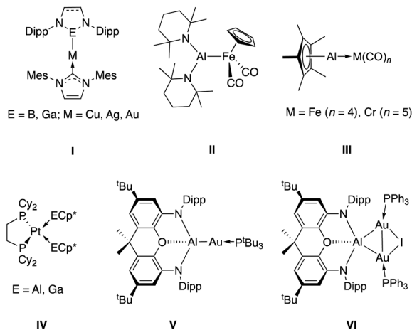
Chart 1 Selected examples of transition metal – group 13 complexes: coinage metal complexes made by metathesis using boryl or gallyl nucleophiles ( I ); 17,18 an Fe–Al bond synthesized from [CpFe(CO) 2 ] − ( II ); 19 transition metal complexes of AlCp* and GaCp* ( II and III ); 20,21 previously communicated aluminium–gold complexes formed from an aluminyl nucleophile and Au(I) electrophiles ( V and VI ). 22
