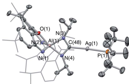
Fig. 4 Molecular structure of 5-Ag in the solid state as determined by X-ray crystallography. Thermal ellipsoids set at the 50% probability level. Hydrogen atoms omitted and {}^1\text{Pr}/{}^t\text{Bu} shown in wireframe for clarity. Key bond lengths (Å) and angles (°): Ag(1)–C(48): 2.118(2), Ag(1)–P(1): 2.3851(6), N(3)–C(48): 1.346(3), N(4)–C(48): 1.345(3).
