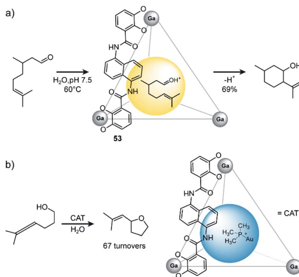
Fig. 24 (a) Prins cyclisation of citronellal catalysed by Raymond's Ga^{III} coordination cage. (b) Encapsulated catalyst Me_3PAu^+ catalyses hydroxyalkylation of alcohol-tethered allenes. Reproduced from ref. 137 with permission from the Royal Society of Chemistry, copyright 2021.
