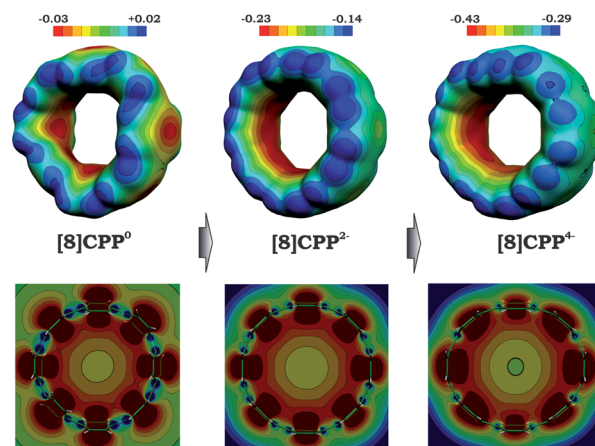
Fig. 7 3D maps (top) and 2D cross-section (bottom) of the molecular electrostatic potential (MEP) for \mathbf{1}^0 , \mathbf{1}^{2-} , and \mathbf{1}^{4-} (PBE0/cc-pVTZ).
