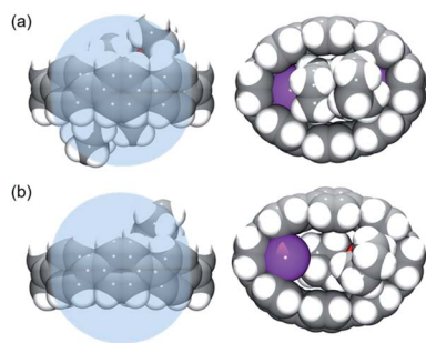
Fig. 4 Comparison of host-guest interactions of \mathbf{1}^{4-} nanohoop in 2 (a) vs. that in ref. 62 (b), side and face views, space-filling models. The internal space is shown as the blue sphere.
