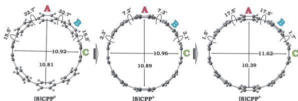
Fig. 5 Optimized geometries along with selected geometrical parameters for \mathbf{1}^0 , \mathbf{1}^{2-} , and \mathbf{1}^{4-} (PBE0/cc-pVTZ).
