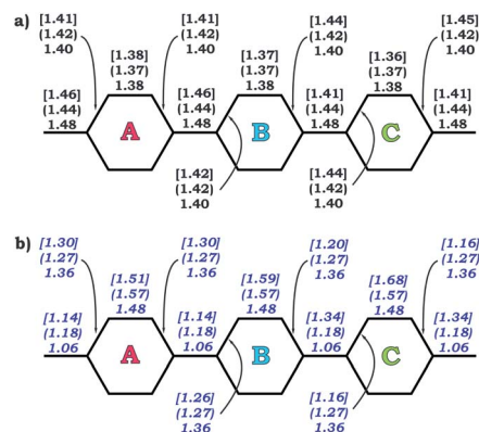
Fig. 6 Selected C-C bond lengths (a) and bond orders (b) calculated for rings A, B, and C (PBE0/cc-pVTZ) in \mathbf{1}^0 , \mathbf{1}^{2-} (round brackets), and \mathbf{1}^{4-} [square brackets].
