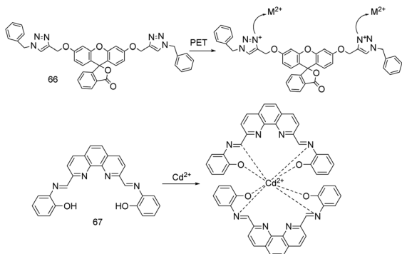
Fig. 24 Proposed sensing mode of probes 66 and 67 with Cd^{2+} .
