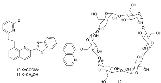
Fig. 4 The structure of probes 10 to 12.
