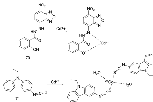
Fig. 26 Proposed binding mode of probes 70 and 71 with Cd^{2+} .
