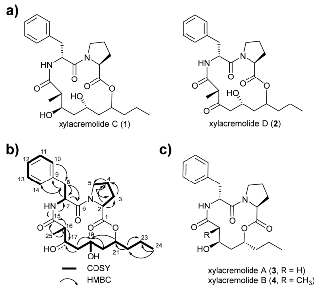
Fig. 2 (a) Structures of isolated xylacremolides C (1) and D (2); (b) representative COSY and HMBC correlation of xylacremolide C (1); (c) structures of previously isolated xylacremolides A (3, R = H) and B (4, R = CH 3 ) from X187.
