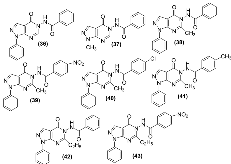
Fig. 12 Chemical structures of selected pyrazolo[3,4-d]pyrimidines (36–43).
