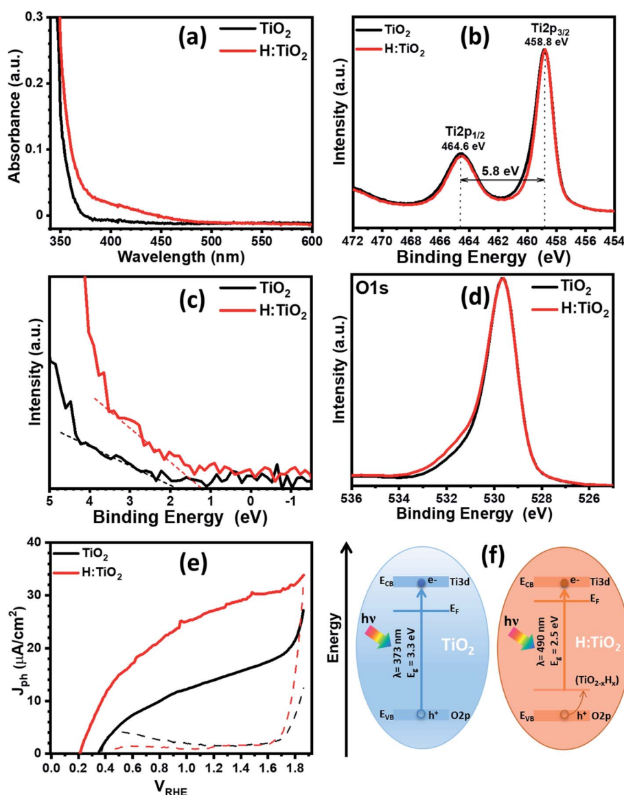
Fig. 5 (a) Optical absorption of pristine and hydrogen treated TiO 2 thin films. (b) Core-level XPS Ti 2p spectra. (c) Valance band spectra of pristine and hydrogen treated TiO 2 . (d) Core-level XPS O 1s spectra. (e) Photocurrent density versus applied potential for pristine and hydrogen treated TiO 2 . (f) Band diagram representation of pristine and hydrogen treated TiO 2 . Both representations were built using experimental data from UV-vis spectroscopy and valance band XPS analysis. Conduction band offset was estimated using band gap and valance band offsets.
