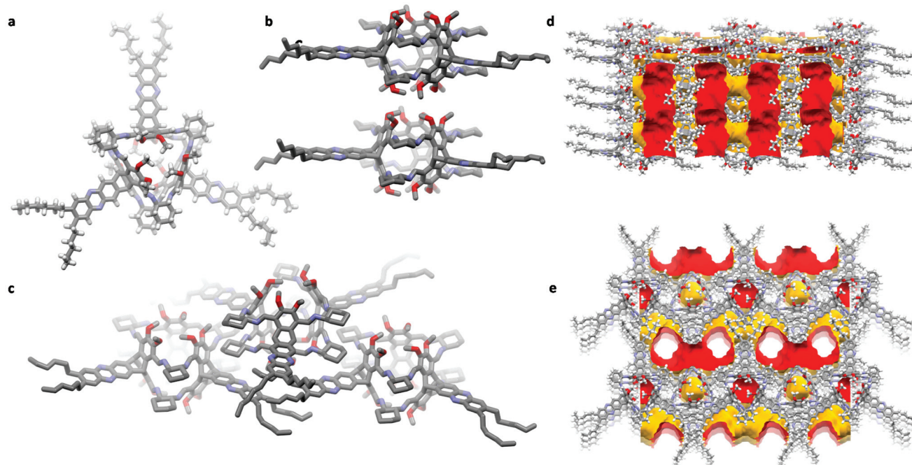
Fig. 4 Single crystal X-ray structure of cage ( R,R )- 9 . (a) single molecule from top; (b) window-to-window packing; (c) packing by \text{CH}\cdots\pi interactions of aromatic phenazine units and aliphatic cyclohexyl ring; (d) and (e) calculated pores with a probe radius of 1.82 \text{\AA} . For (b) and (c) hydrogen atoms have been omitted for clarity. In (d) and (e) the red surface is the solvent accessible surface and yellow the inaccessible surface.
