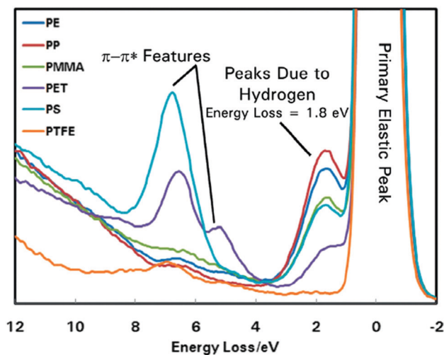
Fig. 18 REELS spectra of polyethylene, polypropylene, poly(methyl methacrylate), polyethylene terephthalate, polystyrene and poly tetrafluoroethylene to evidence the changing peak intensity at \sim 1.8 eV with differing H concentration. Reprinted (adapted) with permission from ref. 391. Copyright (2013) Thermo Scientific.
