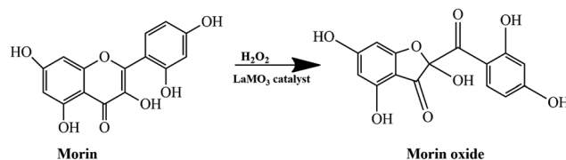
Scheme 1 Oxidation of morin to morin oxide by \text{H}_2\text{O}_2 over \text{LaMO}_3 ( \text{M} = \text{Co}, \text{Cr}, \text{Fe}, \text{Ni}, \text{Mn}, \text{Cu}, \text{Zn} ) perovskites.
