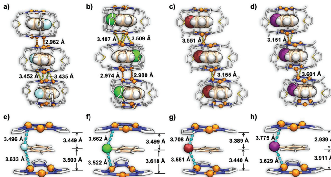
Fig. 1 Crystal structures of (a) 1 ⊃ Ph-F, (b) 1 ⊃ Ph-Cl, (c) 1 ⊃ Ph-Br, and (d) 1 ⊃ Ph-I, showing the Cu 3 L 6 cage units in one packed column with intermolecular Cu...Cu distances of 2.962, 3.452 and 3.435 Å in 1 ⊃ Ph-F, 3.407, 3.509, 2.974 and 2.980 Å in 1 ⊃ Ph-Cl, 3.551 and 3.155 Å in 1 ⊃ Ph-Br, and 3.151 and 3.601 Å in 1 ⊃ Ph-I, respectively (Cu(I) ions, cage hosts 1 , and halobenzene guests are shown as the ball, line and space-filling model, respectively; hydrogen atoms in cage hosts 1 are omitted for clarity; C, N, S, and Cu atoms in the cage are shown in gray, blue, yellow, and orange colours, respectively; C, H, F, Cl, Br and I atoms in the guests are shown in wheat, white, light cyan, green, brown and purple colours, respectively); CTC-guest-CTC structures of (e) 1 ⊃ Ph-F, (f) 1 ⊃ Ph-Cl, (g) 1 ⊃ Ph-Br, and (h) 1 ⊃ Ph-I, showing intermolecular Cu...X distances of 3.496 and 3.633 Å in 1 ⊃ Ph-F, 3.662 and 3.522 Å in 1 ⊃ Ph-Cl, 3.778 and 3.551 Å in 1 ⊃ Ph-Br, and 3.775 and 3.629 Å in 1 ⊃ Ph-I, respectively (Cu(I) ions, halogen atoms, CTC units, and guests are shown as the ball and line model, respectively).
