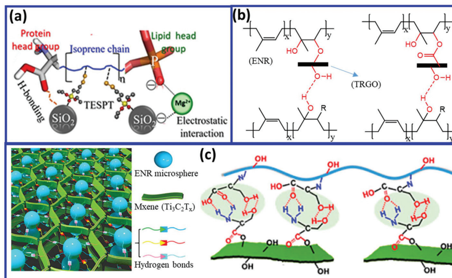
Fig. 19 (a) Schematic representation of the electrostatic interaction and hydrogen bonding in the NR/ \text{SiO}_2 composites. 113 (b and c) Hydrogen bonding in the ENR/TRGO and serine-modified ENR/Mxene composites. 114,115 Reproduced from ref. 113 with permission from American Chemical Society, copyright 2019. Reproduced from ref. 114 with permission from American Chemical Society, copyright 2020. Reproduced from ref. 115 with permission from American Chemical Society, copyright 2020.
