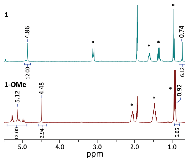
Fig. 2 ^1\text{H} NMR spectra of complexes 1 (top, blue) and 1-OMe (bottom, red) collected in \text{CD}_3\text{CN} at 21 °C. Formation of the alkylated species 1-OMe is indicated by the appearance of a singlet peak belonging to the bridging methoxide ligand at 4.48 ppm, along with a downfield shift of the signal corresponding to the terminal methyl group of the capping triol ligand (0.74 and 0.92 ppm for 1 and 1-OMe respectively). Additionally, the singlet peak corresponding to the methylene group of the parent cluster 1 (4.86 ppm) splits into a multi-peak pattern upon formation of the alkylated species 1-OMe (peaks centred at 5.12 ppm). Peaks labelled with * indicate signals belonging to the cations [\text{Bu}_4\text{N}]^+ and [\text{Bu}_4\text{P}]^+ for 1 and 1-OMe respectively. Peak assignments for alkylated species can be found in Fig. S1 and S7† for 1-OMe and 2-OMe respectively.
