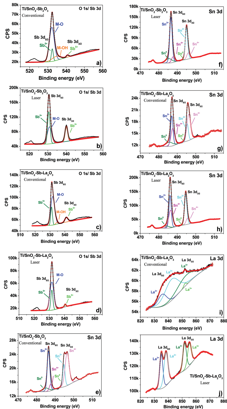
Fig. 4 High-resolution XPS spectrum of O 1s/Sb 3d, Sn 3d and La 3d for \text{Ti}/\text{SnO}_2\text{-Sb}_2\text{O}_5 electrodes (a and e) conventional, (b and f) laser and \text{Ti}/\text{SnO}_2\text{-Sb-LazO}_3 electrodes. (c, g and i) Conventional and (d, h, and j) laser.
