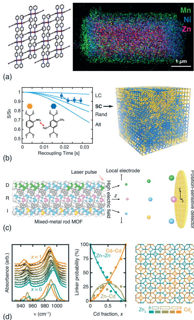
Fig. 3 Determining compositional correlations in compositionally disordered MOFs. (a) STEM-EDX images of transition-metal segregation in the mixed-metal Zn/Ni/Mn/CID-5 \gamma MOF. 58 Adapted from ref. 58 with permission from the American Chemical Society. (b) REDOR-NMR decay curves are sensitive to the degree of clustering/anticlustering of individual linkers in mixed-linker MOFs (LC = large clusters, SC = small clusters, Alt = alternating). 54 Adapted from ref. 54 with permission from the American Association for the Advancement of Science. (c) Atom probe tomography allows the sequencing of metal-oxide rods in multivariate MOF-74. 62 Here the method is shown to differentiate ‘duplicate’ (D), random (R), and ‘insertion’ (I) sequences. Adapted from ref. 62 with permission from the American Association for the Advancement of Science. (d) The in-plane methylimidazolate (mIm) stretching region of the IR spectra of mixed-metal (Zn/Cd) ZIF-8 derivatives is sensitive to the relative populations of Zn–mIm–Zn, Zn–mIm–Cd and Cd–mIm–Cd linkages. These populations can be extracted using non-negative matrix factorisation and used to derive models of the Zn/Cd distribution, which is found to involve clustering. 63 Note the greater-than-statistical population of Zn 4 /Cd 4 four-rings (experimental Zn n Cd 4-n populations as solid bars; statistical populations as open bars). Adapted from ref. 63 with permission from the Royal Society of Chemistry.
