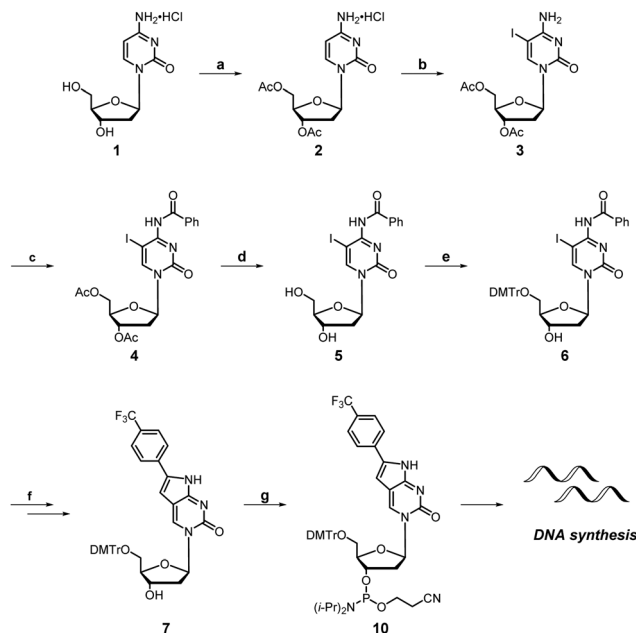
Scheme 1 Synthesis of FPdC and FPdC -containing DNA. Reagents and conditions: (a) \text{CH}_3\text{COCl} , \text{AcOH} , \text{CHCl}_3 , 50–60 °C, 3 days; (b) \text{I}_2 , \text{HIO}_3 , \text{AcOH} , 40 °C, 24 h; (c) \text{Bz}_2\text{O} , pyridine, 85 °C, 3 h; (d) \text{K}_2\text{CO}_3 , \text{MeOH} , r.t., 1 h; (e) \text{DMTrCl} , pyridine, r.t., 4 h; (f) 4-ethynyl trifluorotoluene, \text{Pd}(\text{PPh}_3)_2\text{Cl}_2 , \text{CuI} , \text{Et}_3\text{N} , \text{THF} , 50–55 °C, 18 h, then \text{Et}_3\text{N} , \text{EtOH} , 55 °C 18 h; (g) (\text{iPr}_2\text{N})_2\text{PO}(\text{CH}_2)_2\text{CN} , \text{DIPA} , \text{CH}_2\text{Cl}_2 , 0 °C to r.t. 1.5 h.
