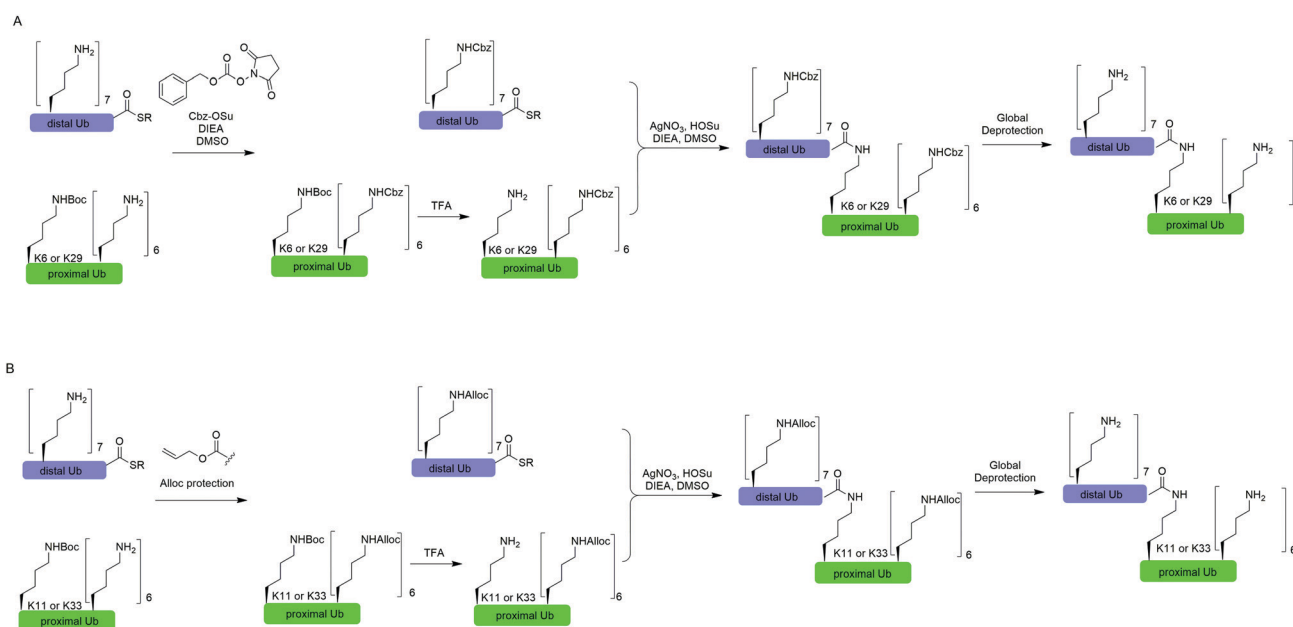
Fig. 7 Silver-mediated chemical ubiquitination to generate K6- and K29-linked diUb (A) and K11- and K33-linked diUb (B).
