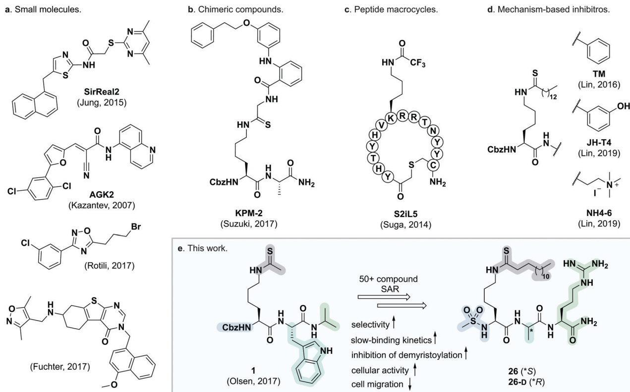
Fig. 1 Representative SIRT2 inhibitors. (a) Heterocyclic small molecule inhibitors. 30,35,46,47 (b) Chimeric lysine mimic KPM-2. 37 (c) Peptide macrocycle S2iL5. 34 (d) Mechanism-based inhibitors based on modified lysine. 24,32,40 (e) Summary of this study.
