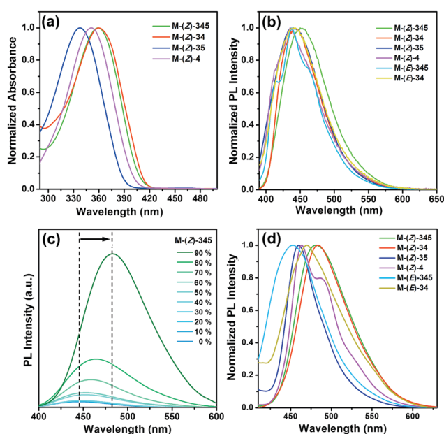
Fig. 4 (a) UV-vis absorption spectra of monomers in CHCl 3 ( 1 \times 10^{-5} mol L -1 ). (b) PL spectra of monomers in CHCl 3 ( 1 \times 10^{-5} mol L -1 ). (c) PL spectra changes of M-(Z)-345 depending on the water fractions in THF. (d) Fluorescence spectra of monomers in the solid state.
