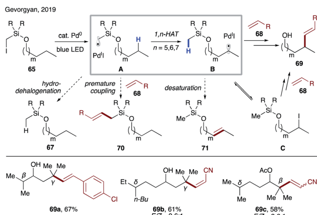
Scheme 17 Radical relay Heck reaction of aliphatic alcohols.
