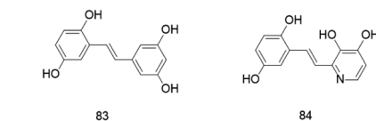
Fig. 13 The chemical structures of inhibitors with diverse mechanisms.
