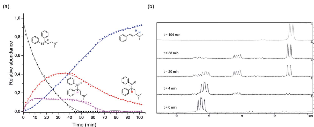
Fig. 2 1 H-NMR mechanistic study of the reaction of 1-H with H 2 O 2 . The graph reported in (a) was obtained by integration of the \alpha -hydrogen signals for the starting material and the two diastereoisomers and the allylic-hydrogens signals for the cinnamylamine in the 1 H-NMR spectra acquired at different time points (• starting material, • R - R (and its enantiomer), • R - S (and its enantiomer) • cinnamylamine 6 ). In (b), representative 1 H-NMR spectra are reported showing the variation over time during the oxidation-reaction of compound 3 , focusing on the region between 4.7 and 3.8 ppm (area of interest to plot the graph; see Fig. S31† for additional spectra).
