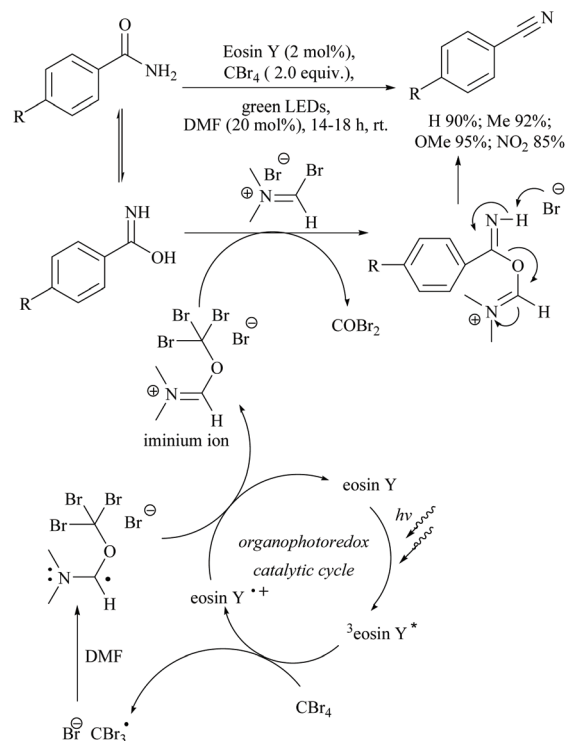
Scheme 53 Organo-photocatalytic dehydration.
