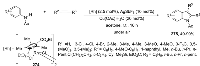
Scheme 219
