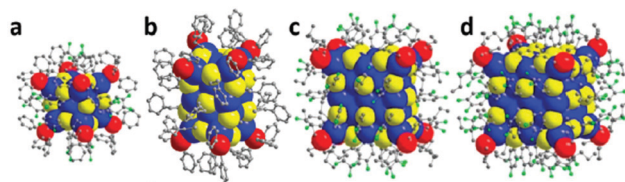
Fig. 5 X-ray structures of Ag cubes: Ag_{14}(SC_6H_3F_2)_{12}(PPh_3)_8 , Ag_{23}(PPh_3)_8-(SC_2H_4Ph)_{18} , Ag_{38}(SPhF_2)_{26}(P^tBu_3)_8 , and Ag_{63}(SPhF_2)_{36}(P^tBu_3)_8 . Adapted with permission from ref. 62. Copyright 2019, Royal Society of Chemistry.
