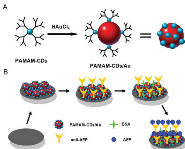
Fig. 4 The schematic diagram of the PAMAM-CDs/Au nanocrystal nanocomposites (A); and fabrication of the PAMAM-CDs/Au nanocomposite-based electrochemical immunosensor (B). Reprinted with permission from ref. 60. Copyright 2013 Elsevier.
