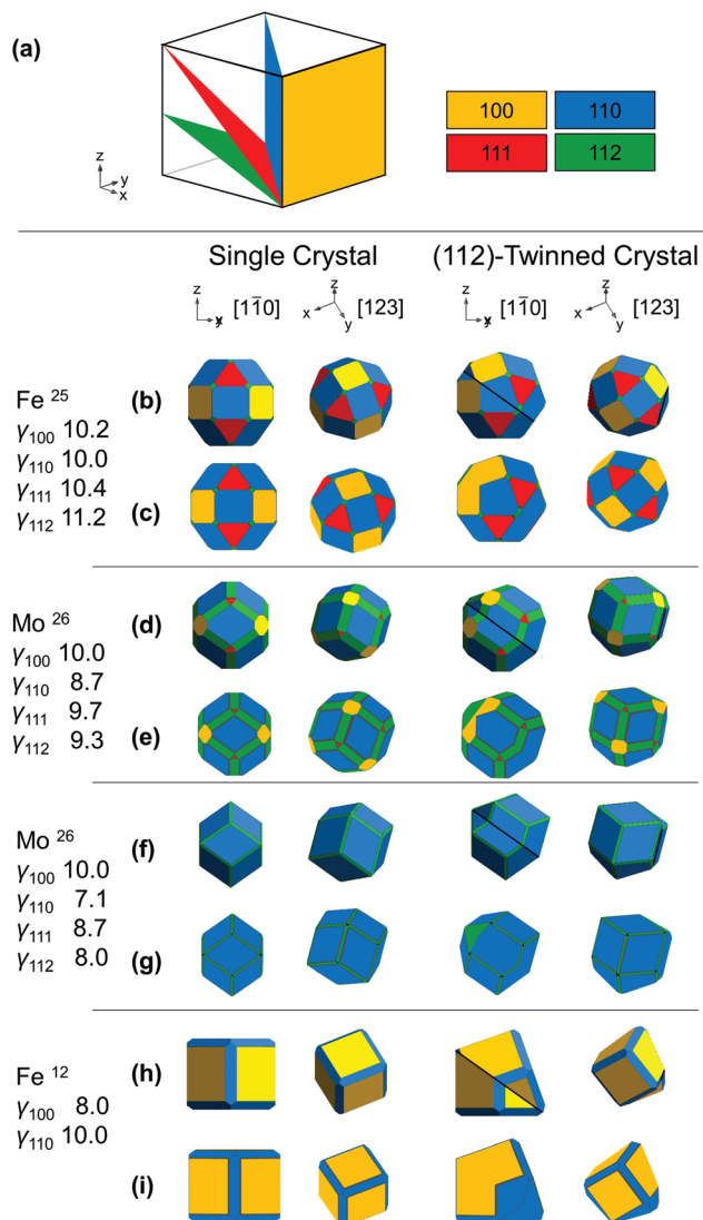
Fig. 1 Shapes of BCC NPs. (a) Dense crystallographic planes in BCC and their color-coding. (b, d, f and h) Analytical thermodynamic and (c, e, g and i) numerical kinetic shapes from the surface energies/growth velocities listed; twin planes are shown as a black line, viewing directions are [110] or [123] ; these and the x , y , z directions refer to the parent crystal, on, for [110] , the bottom left of and, for [123] , behind the crystal.
