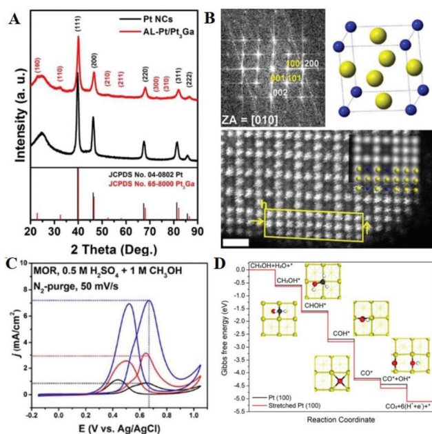
Fig. 3 (A) XRD patterns of XC-72 supported \text{Pt}_3\text{Ga}/\text{Pt} and Pt nanocrystal samples. (B) FFT pattern of the \text{Pt}_3\text{Ga}/\text{Pt} ; the unit cell of the intermetallic \text{Pt}_3\text{Ga} phase, yellow and blue spheres represent Pt and Ga atoms, respectively; enlarged high-resolution HAADF-STEM images. (C) CVs of three catalysts in 1 M methanol + 0.5 M \text{H}_2\text{SO}_4 solution at a sweep rate of 50 mV \text{s}^{-1} . (D) Calculated reaction pathways of the MOR on unstrained Pt (100) and stretched Pt (100) surfaces at pH = 0.25, U = 0.88 V with respect to the RHE. The insets show the optimized structures of intermediates (Pt: yellow, C: black, O: red, H: white). Reproduced with permission from ref. 96. Copyright 2018, American Chemical Society.
