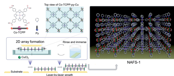
Fig. 7 Schematic illustration of fabrication method of NAFS-1. Reproduced with permission. 90 Copyright©2010 Nature Publishing Group.
